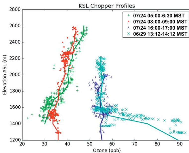
FIG. 5. Vertical profiles of \text{O}_3 from the KSL-TV news helicopter from 29 Jun and 24 Jul 2015. Individual measurements (dots), with best fit (solid line), are marked.
